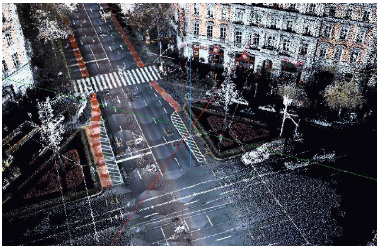
Oktogon square in Budapest, laser scanned by RODIS (Source: Budapest Közút/Budapest Road Management)
